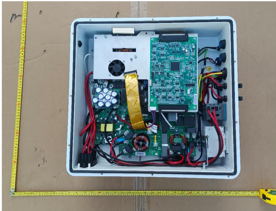
Internal view of inverter for AF6K-ASL
